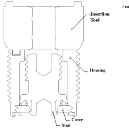
Cross section of IVB fastener with insertion tool
